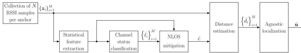
Fig. 1. Block diagram of the proposed localization approach for a generic observation window.
